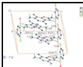
Fig. 2. A view of the C—H...O and C—H... \pi interactions (dotted lines) in the crystal structure of the title compound [symmetry codes: (i) x - 1, y, z ; (ii) -x + 1, -y + 1, -z + 1 ; (iii) x + 1, y, z ]
